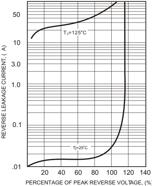
FIG.4-TYPICAL REVERSE CHARACTERISTICS
